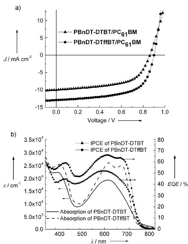
Figure 2. a) Characteristic J – V curves for the BHJ solar cells derived from PBnDT-DTffBT (circle) and PBnDT-DTBT (triangle) under 1 Sun condition (100 mW cm -2 ). b) IPCE and absorption spectra for the BHJ devices derived from PBnDT-DTffBT and PBnDT-DTBT.
